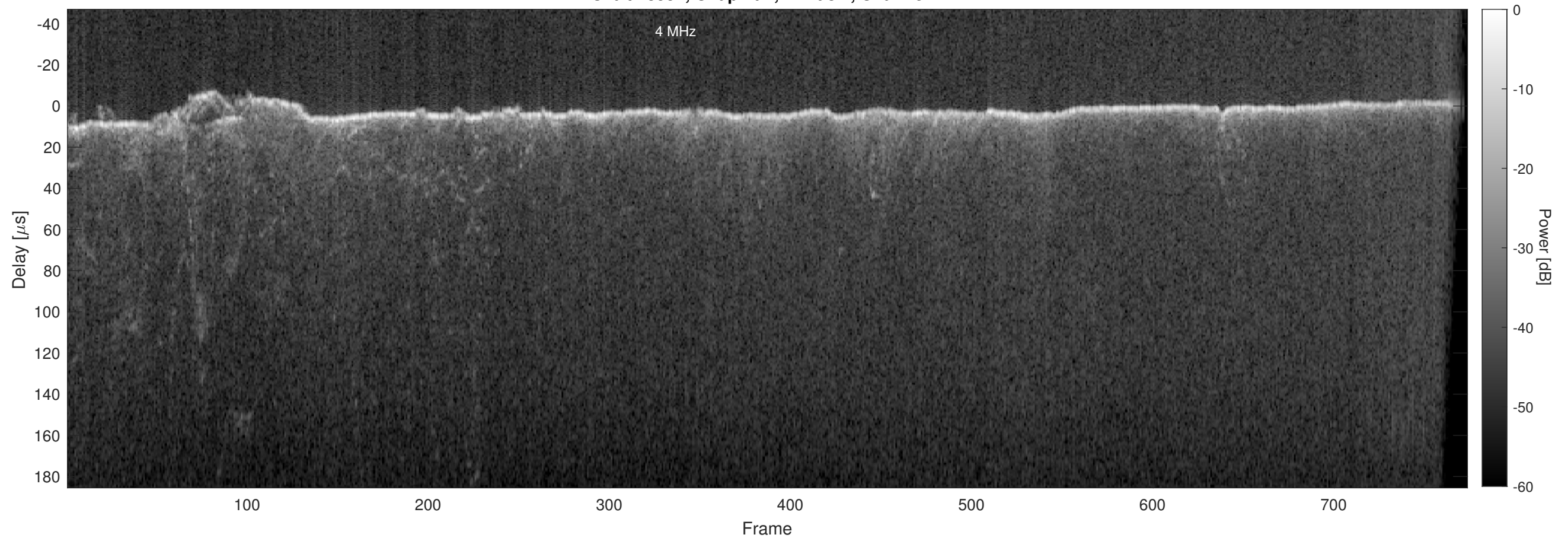
Orbit 18557, Chapman, Window, Channel 2
