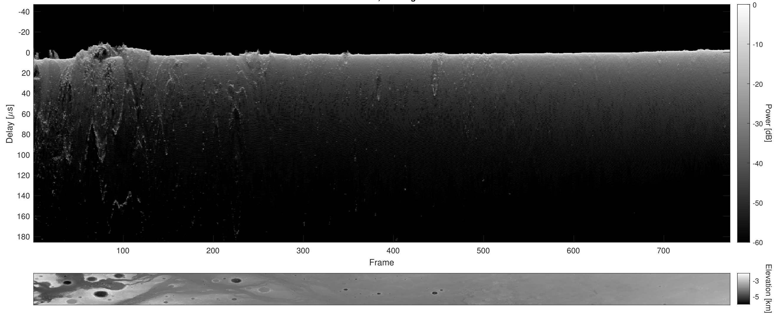
Orbit 18557, Cluttergram
