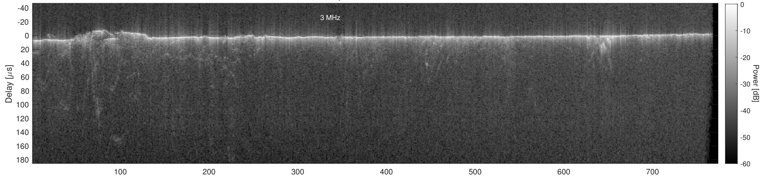
Orbit 18557, Cluttergram
