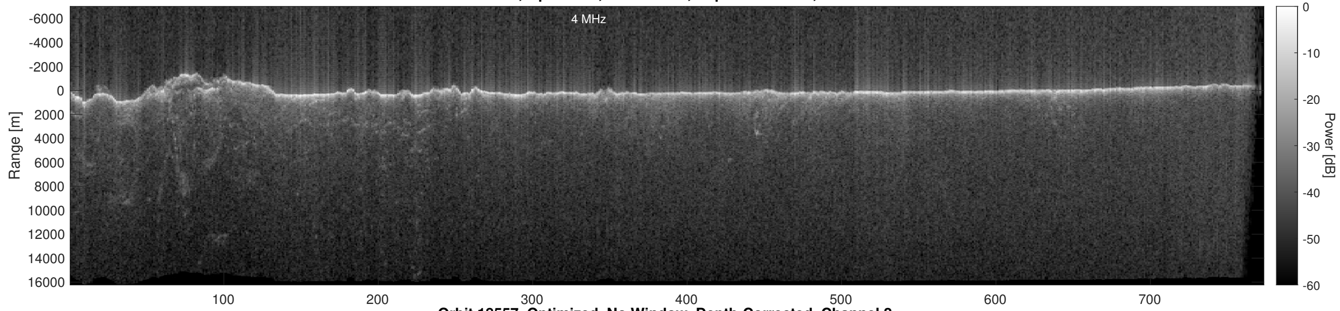
Orbit 18557, Optimized, No Window, Depth-Corrected, Channel 2
