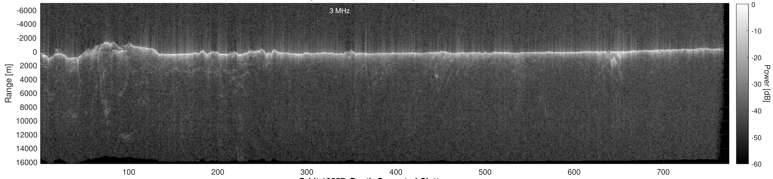
Orbit 18557, Depth-Corrected Cluttergram
