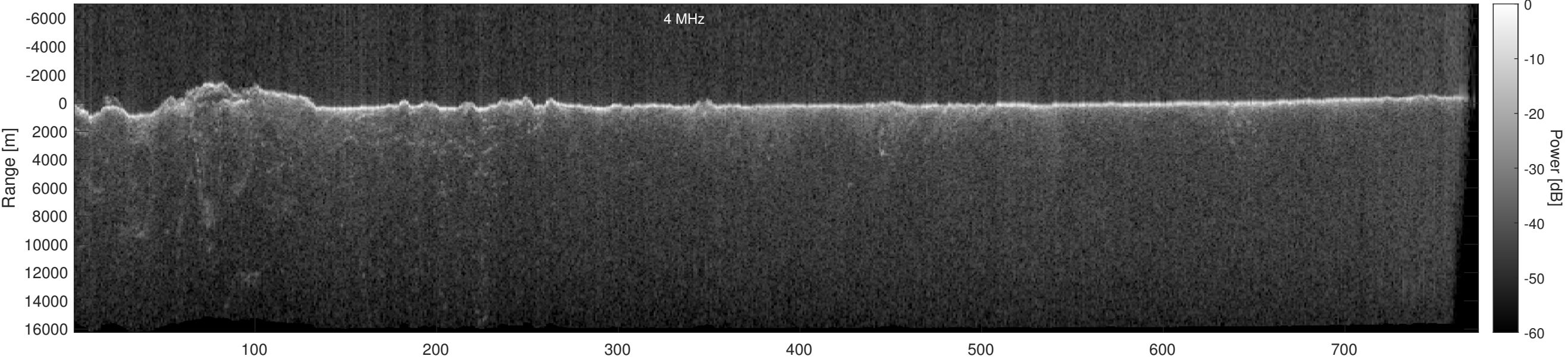
Orbit 18557, Optimized, Window, Depth-Corrected, Channel 2
