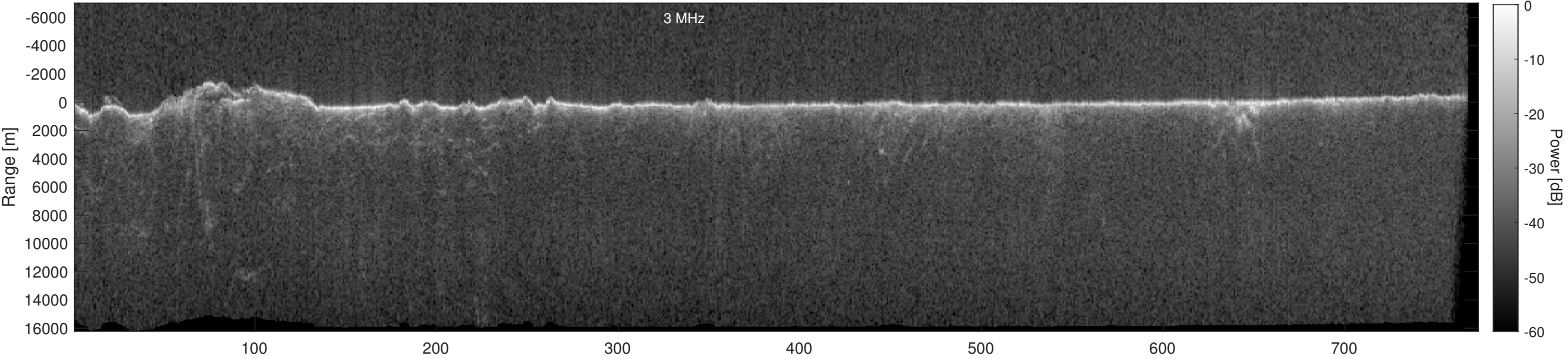
Orbit 18557, Depth-Corrected Cluttergram
