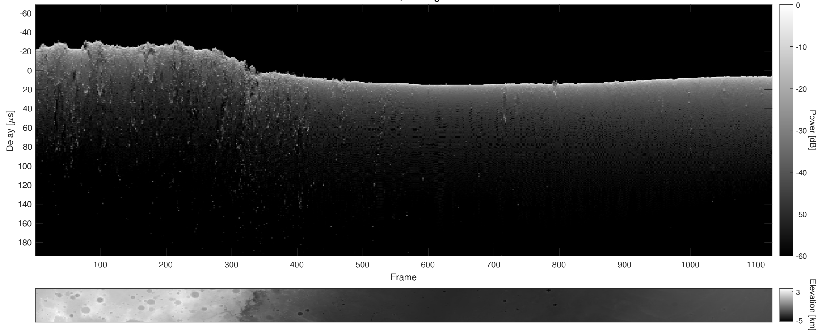
Orbit 18559, Cluttergram
