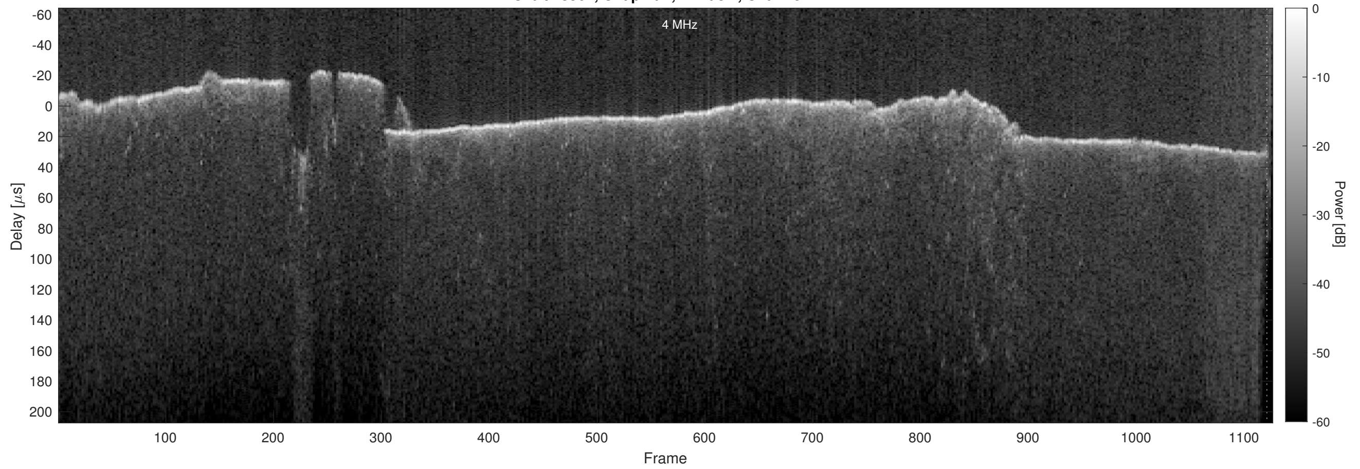
Orbit 18561, Chapman, Window, Channel 2
