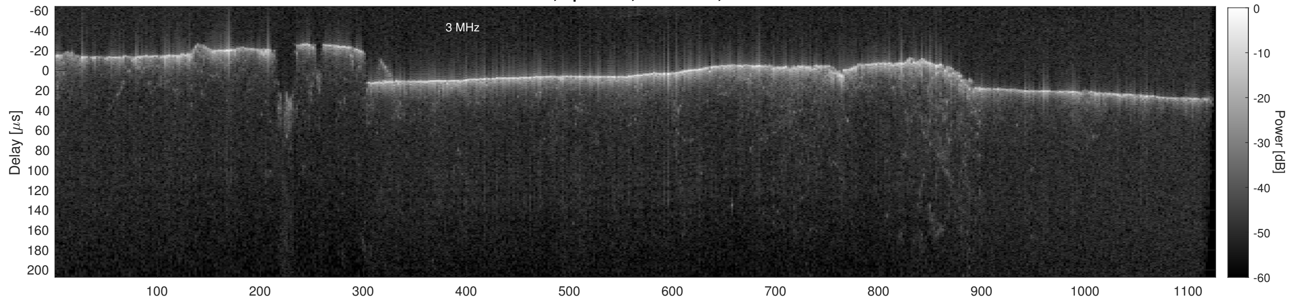
Orbit 18561, Cluttergram
