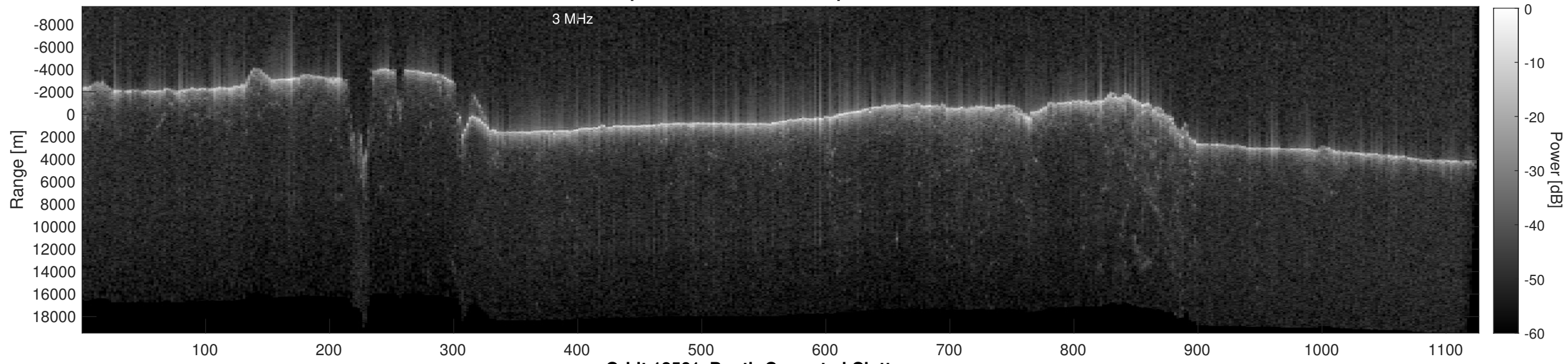
Orbit 18561, Depth-Corrected Cluttergram
