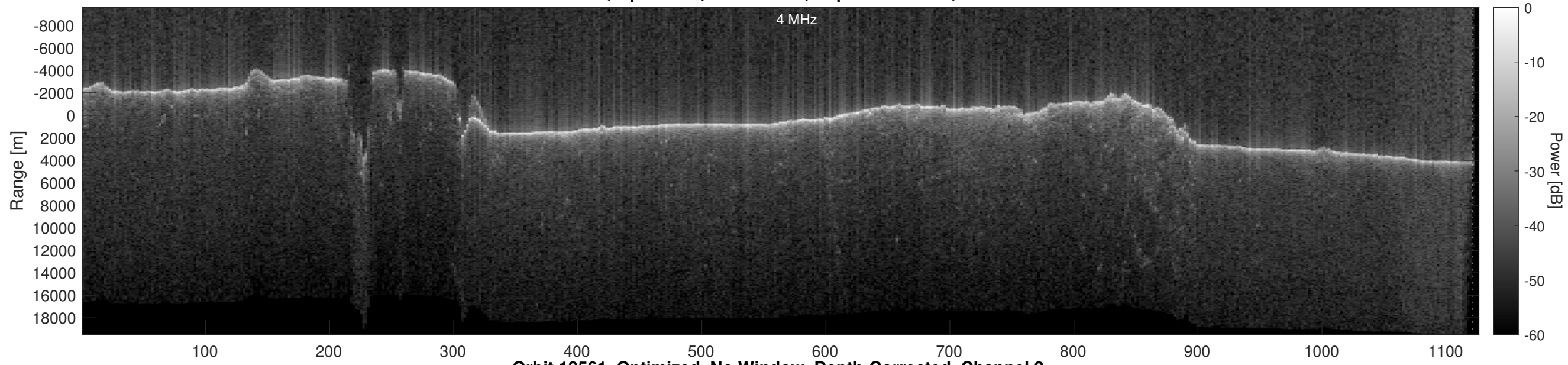
Orbit 18561, Optimized, No Window, Depth-Corrected, Channel 2
