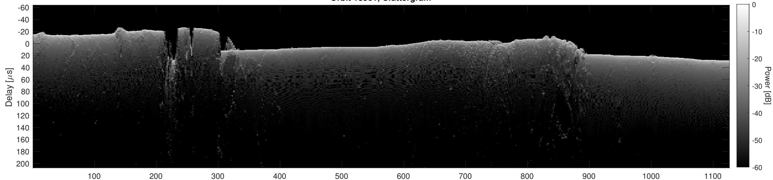
Orbit 18561, Cluttergram
