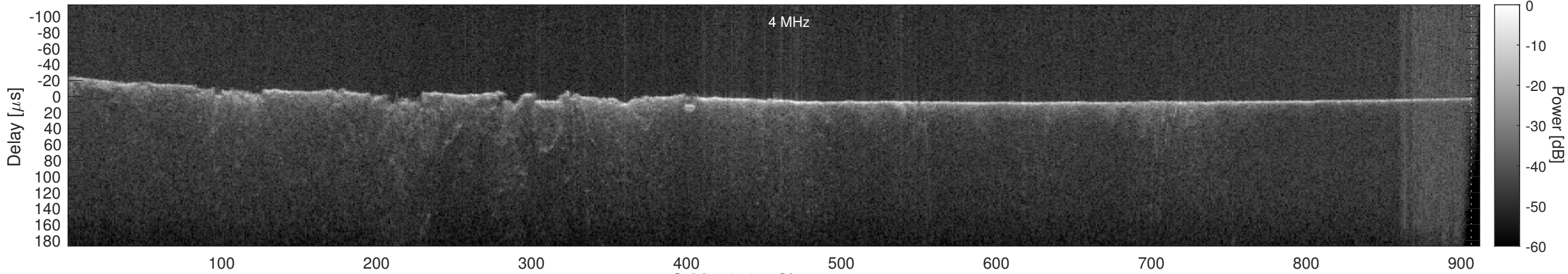
Orbit 18564, Cluttergram
