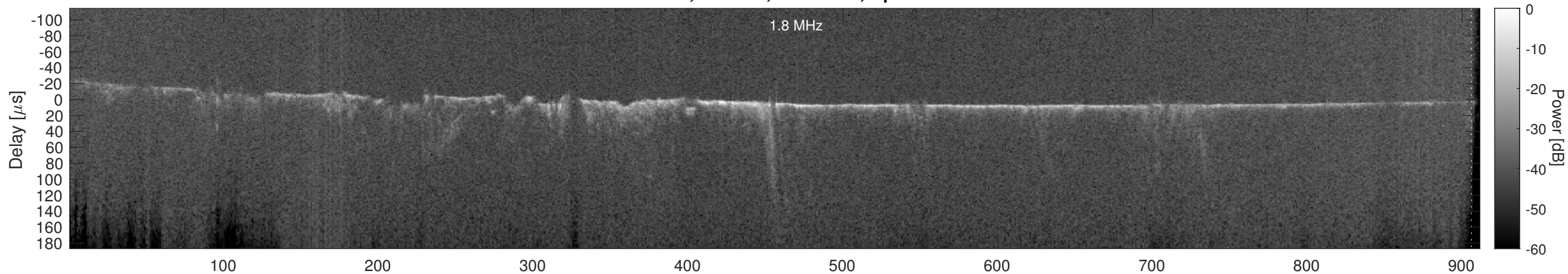
Orbit 18564, Cluttergram
