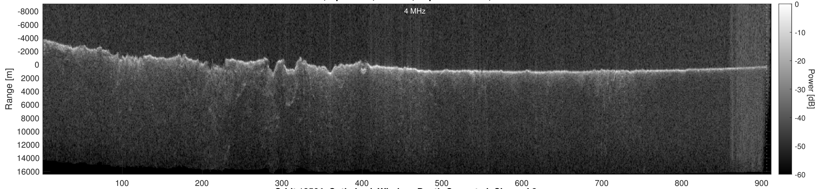
Orbit 18564, Optimized, Window, Depth-Corrected, Channel 2
