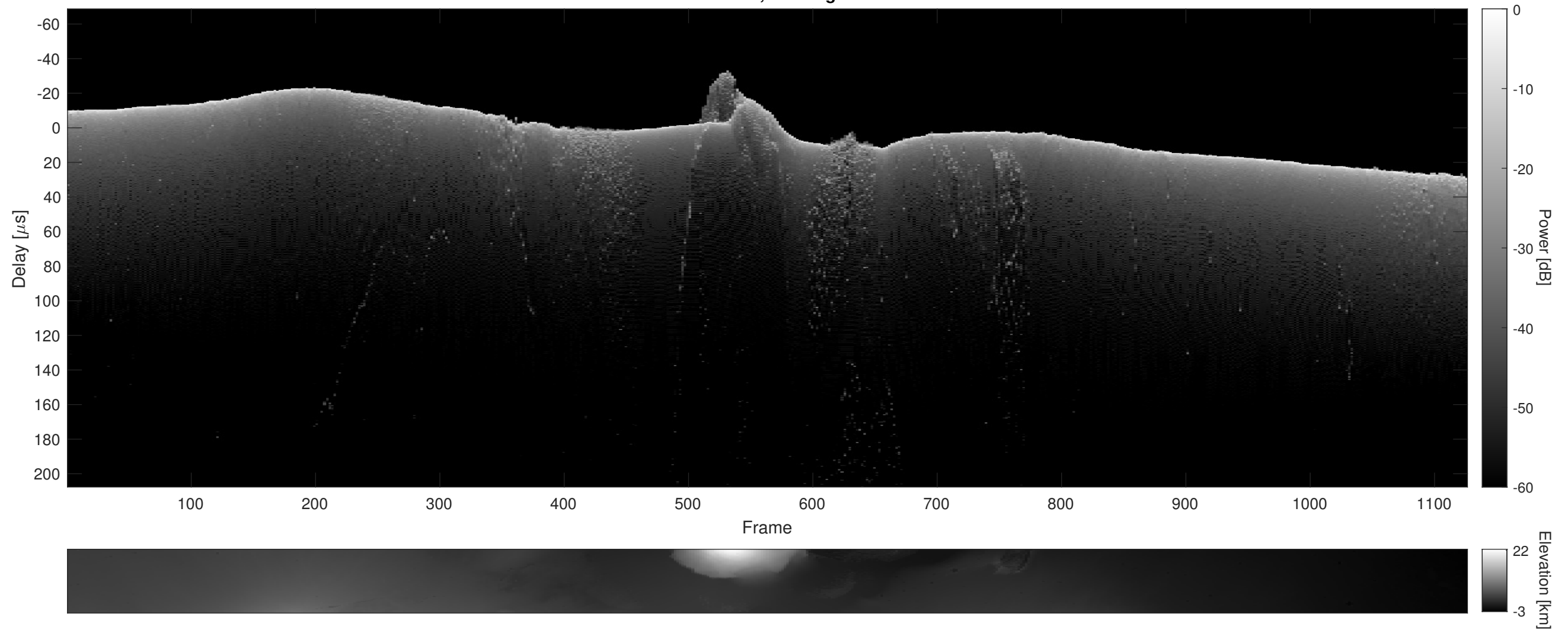
Orbit 18565, Cluttergram
