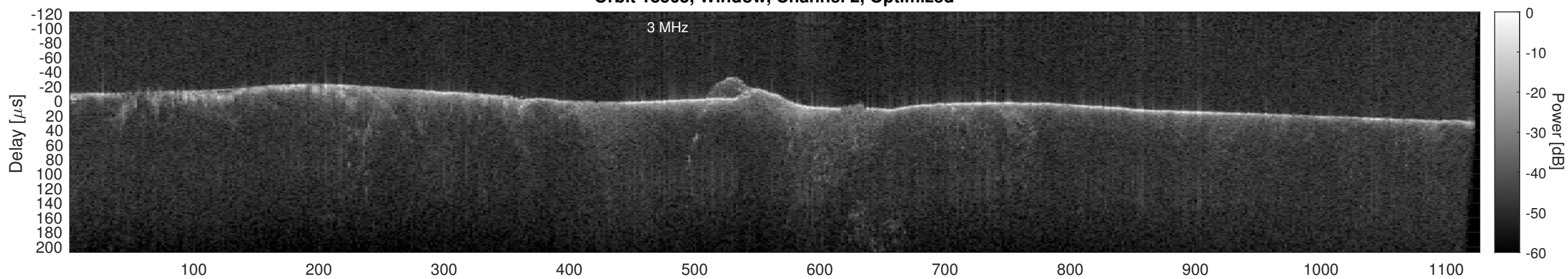
Orbit 18565, Cluttergram
