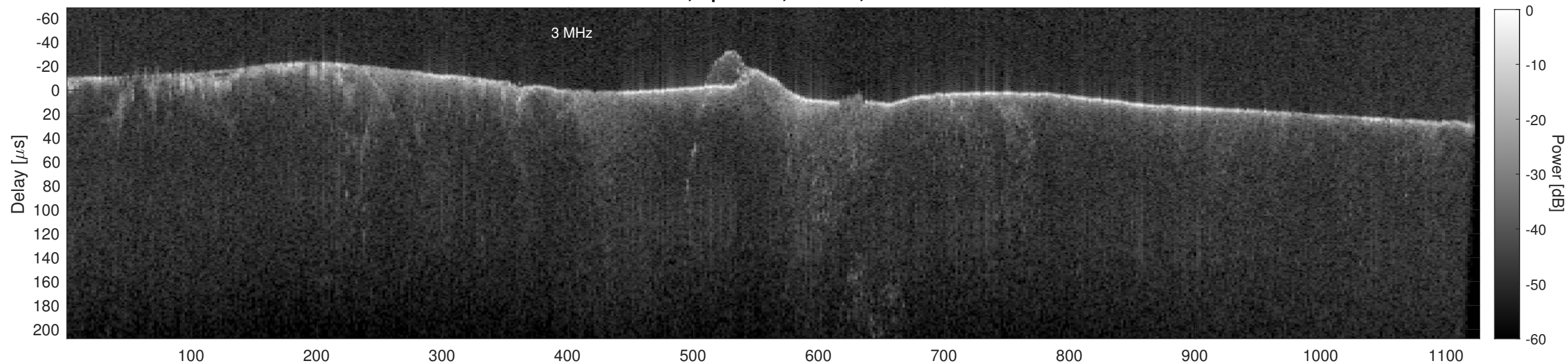
Orbit 18565, Cluttergram
