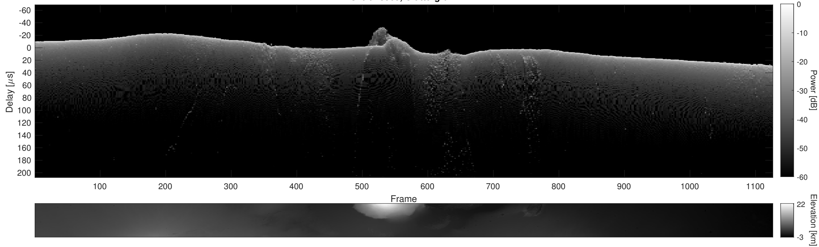
Orbit 18565, Cluttergram
