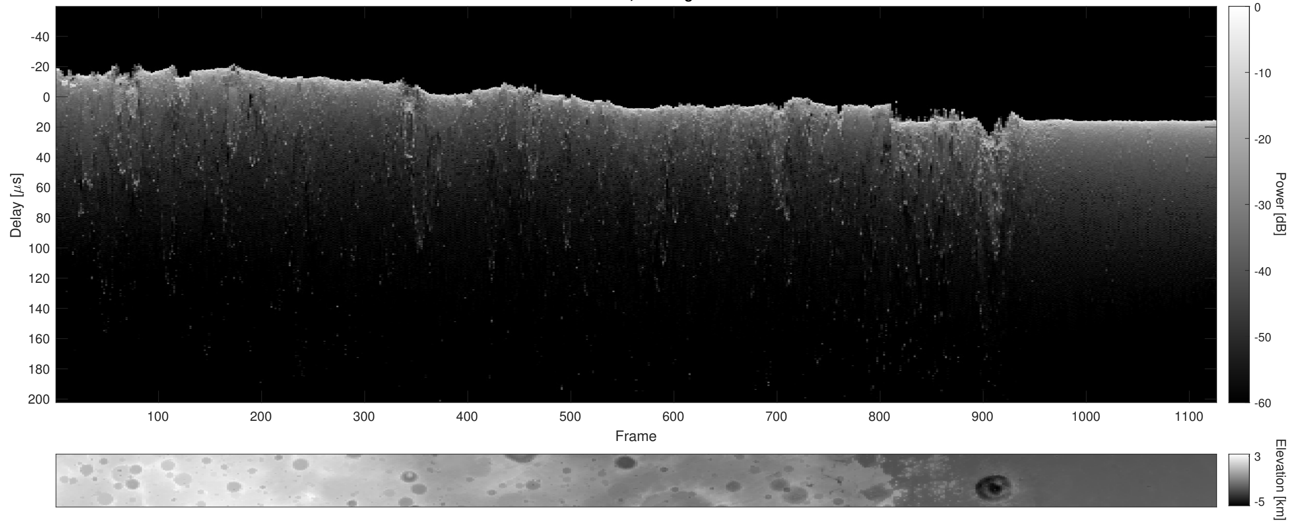
Orbit 18567, Cluttergram
