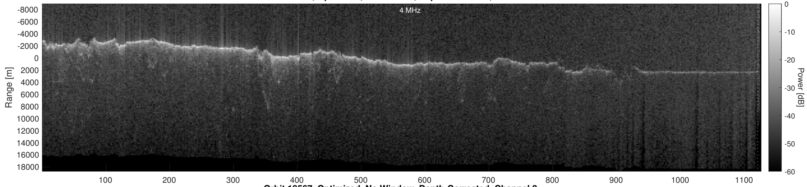
Orbit 18567, Optimized, No Window, Depth-Corrected, Channel 2
