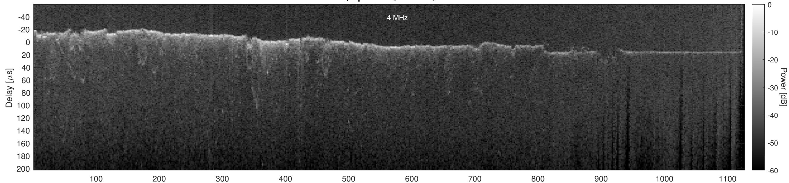
Orbit 18567, Optimized, Window, Channel 2
