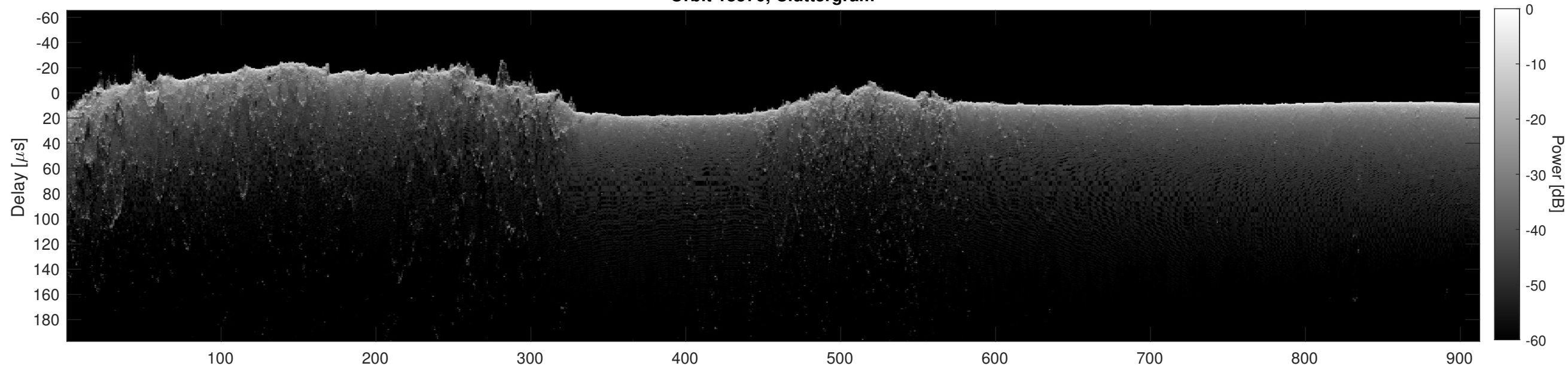
Orbit 18570, Cluttergram
