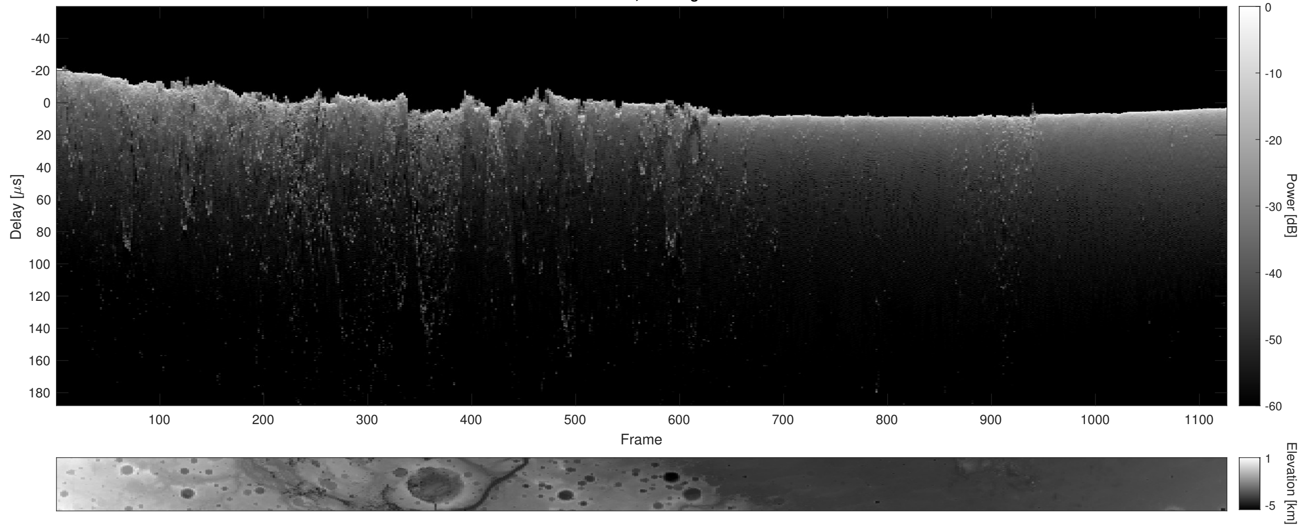
Orbit 18571, Cluttergram
