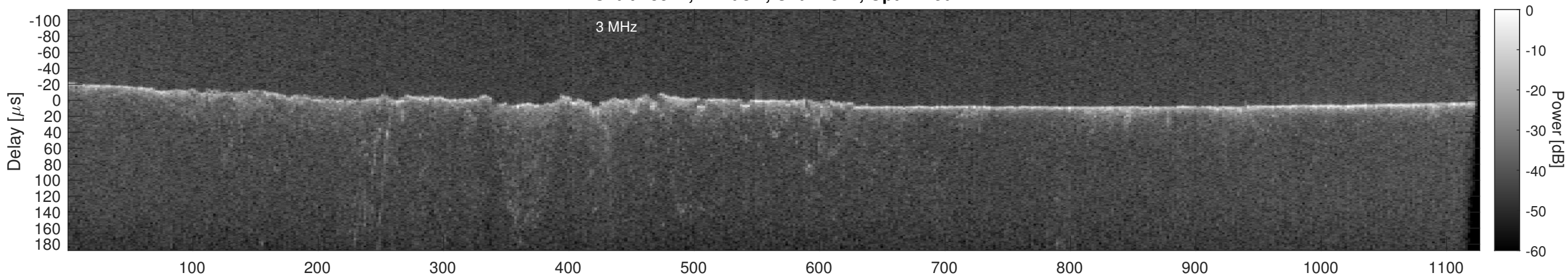
Orbit 18571, Cluttergram
