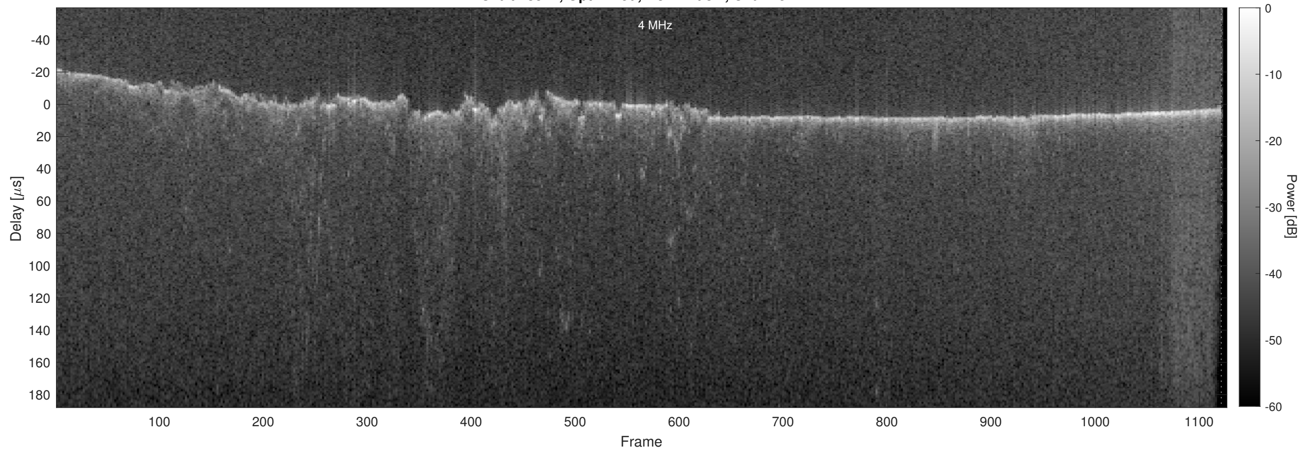
Orbit 18571, Optimized, No Window, Channel 2
