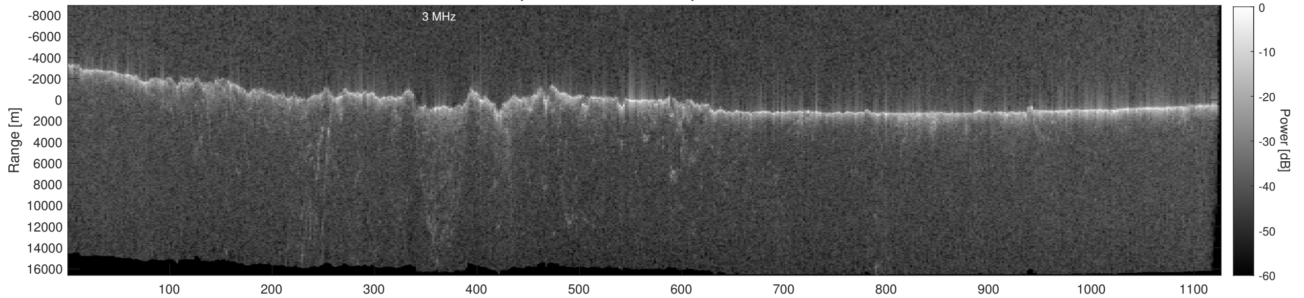
Orbit 18571, Depth-Corrected Cluttergram
