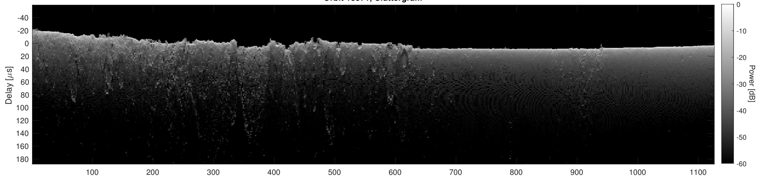
Orbit 18571, Cluttergram
