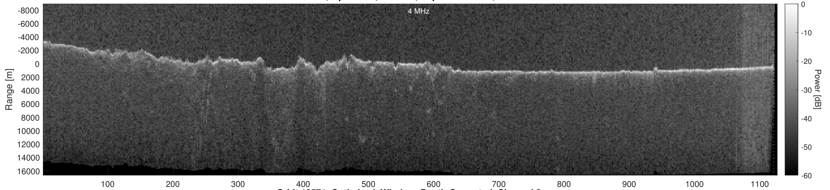
Orbit 18571, Optimized, Window, Depth-Corrected, Channel 2
