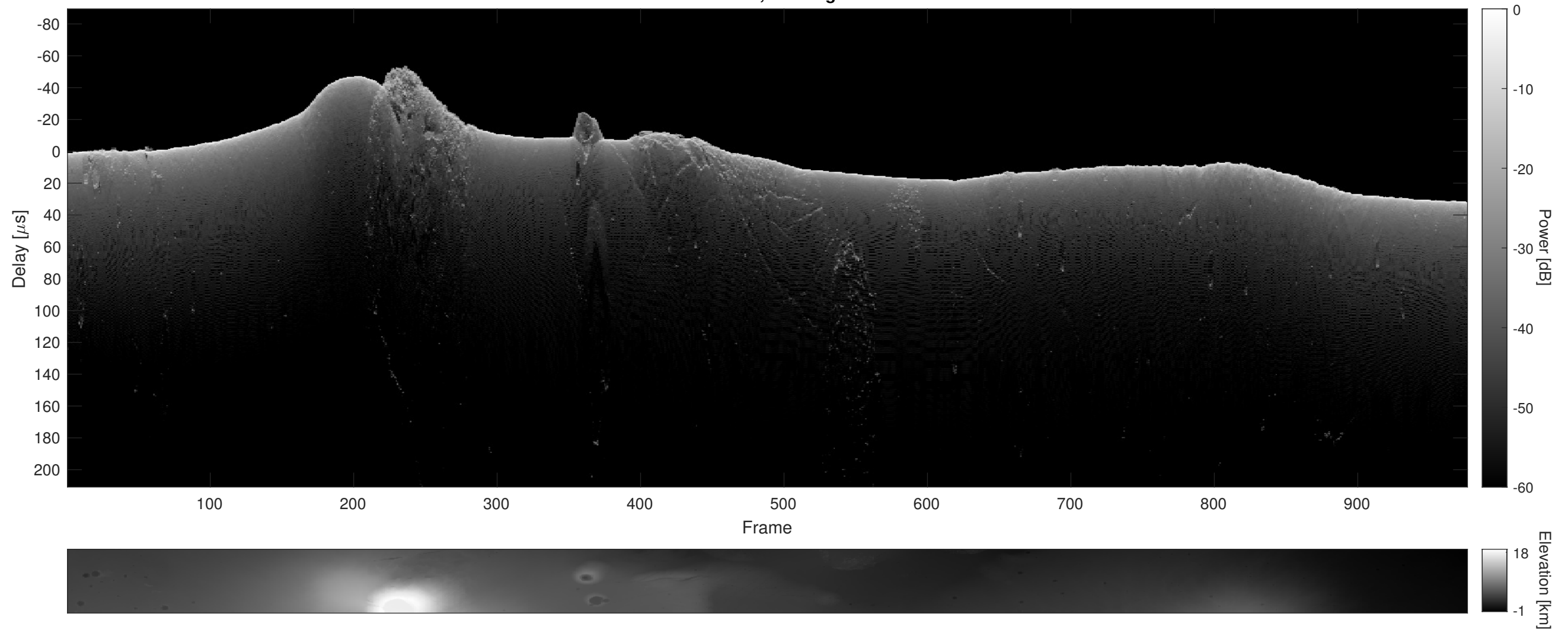
Orbit 18572, Cluttergram
