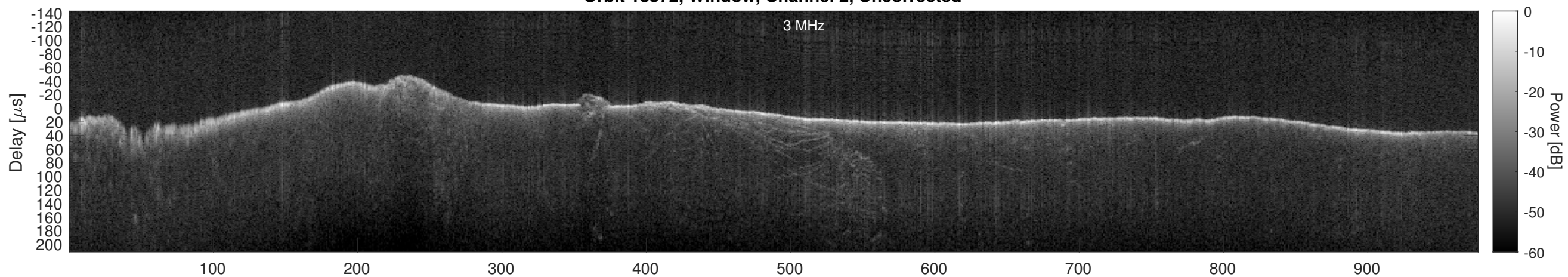
Orbit 18572, Window, Channel 2, Chapman
