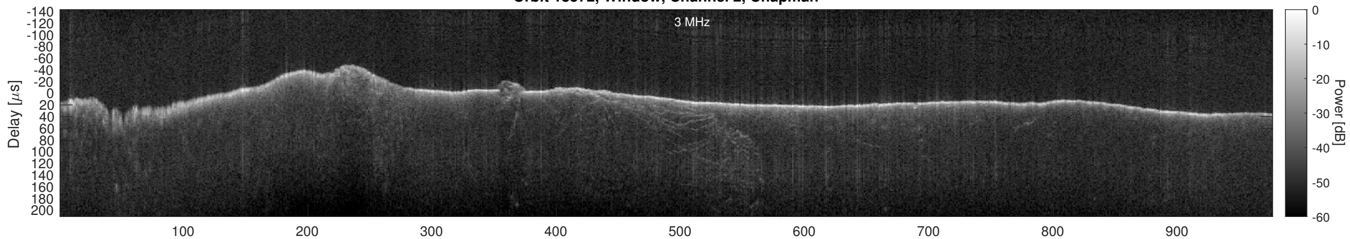
Orbit 18572, Window, Channel 2, Optimized
