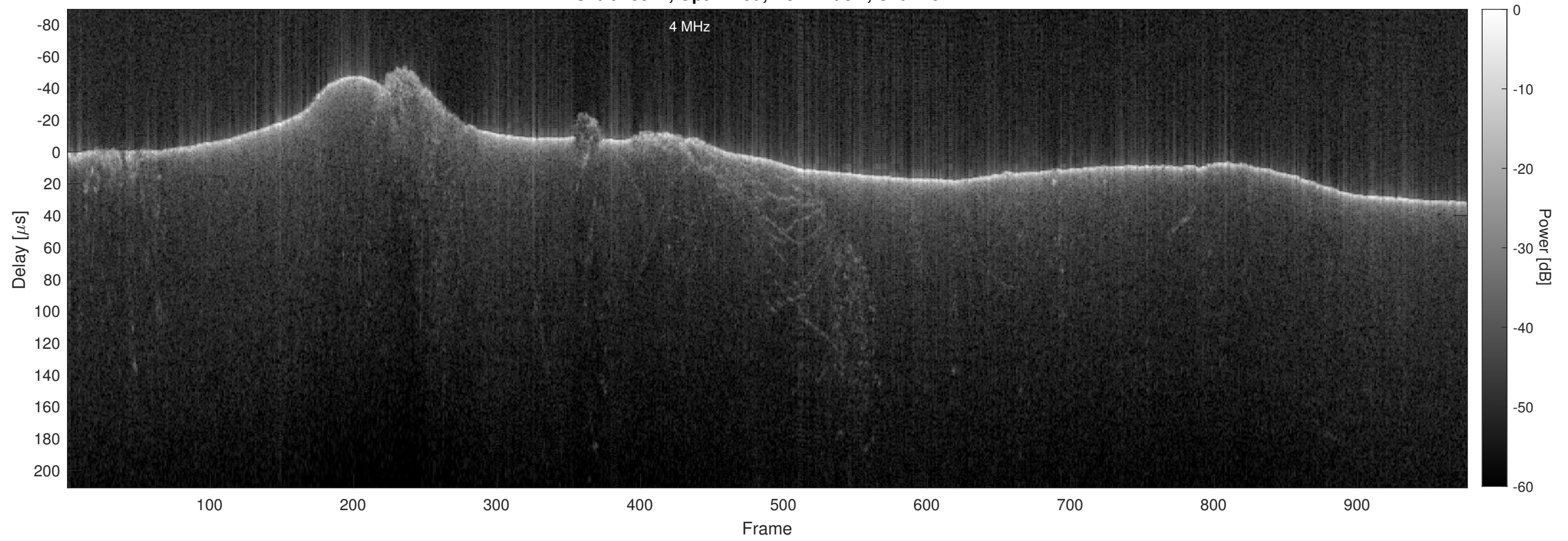
Orbit 18572, Optimized, No Window, Channel 2
