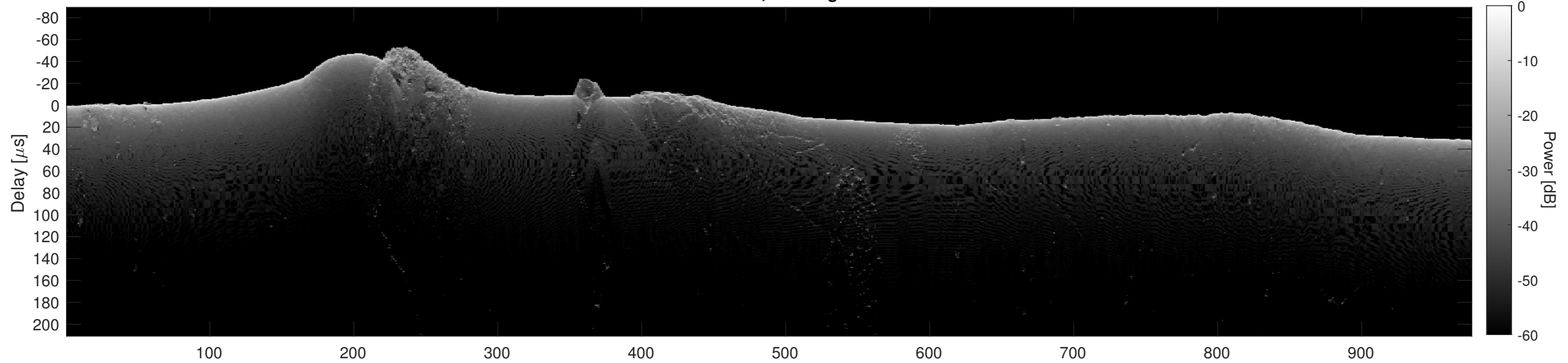
Orbit 18572, Cluttergram
