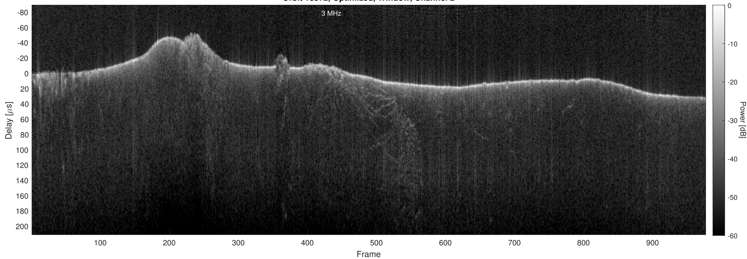
Orbit 18572, Optimized, Window, Channel 2
