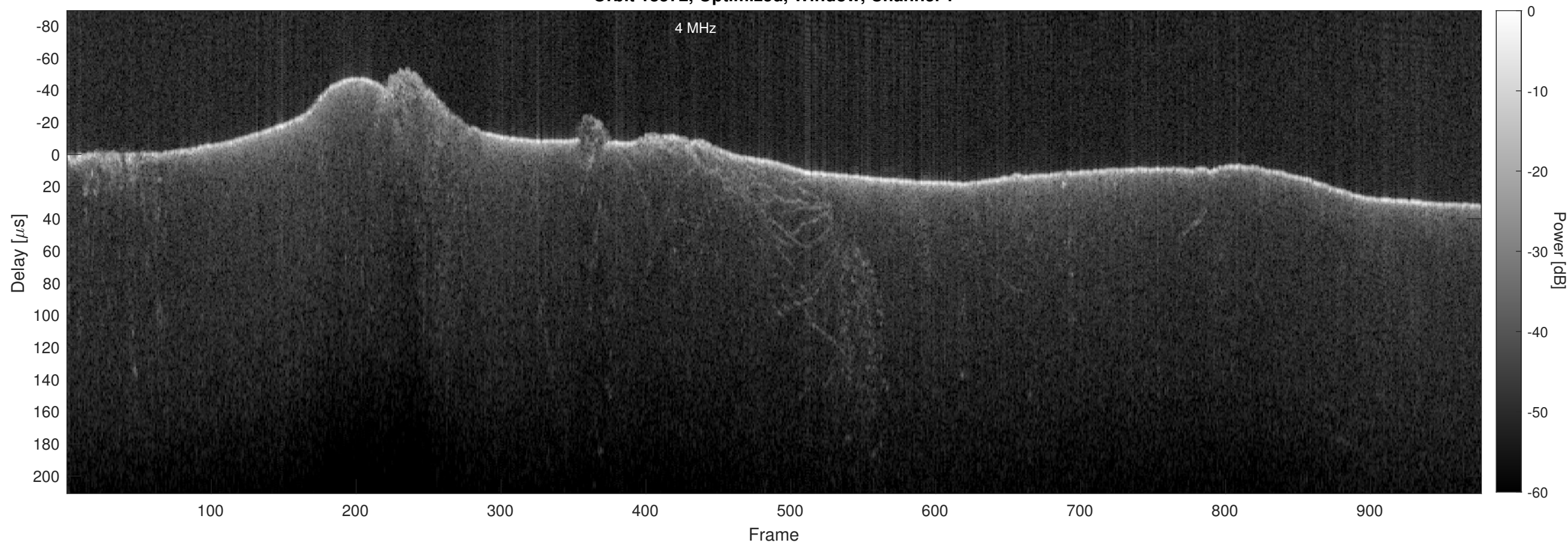
Orbit 18572, Optimized, Window, Channel 2
