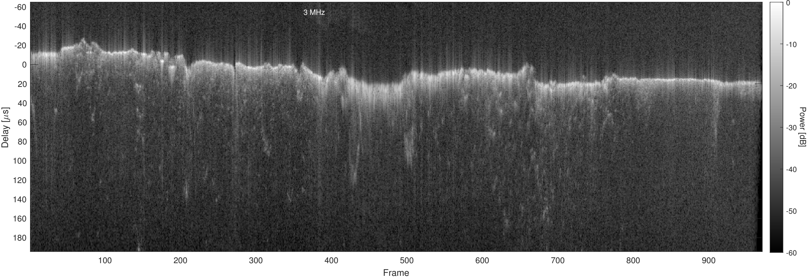
Orbit 18574, Chapman, No Window, Channel 2
