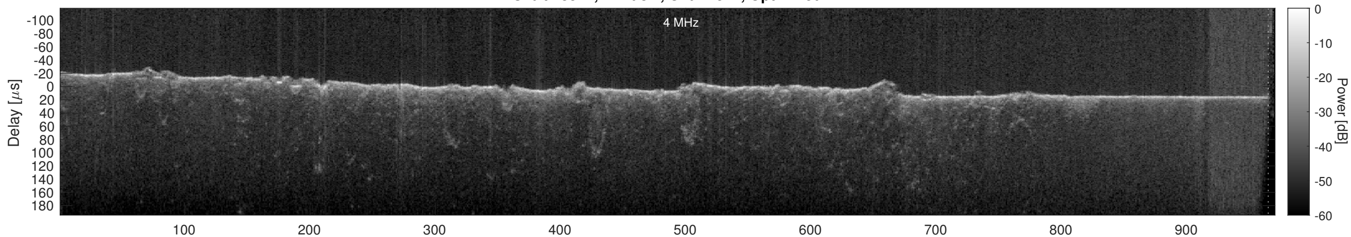
Orbit 18574, Cluttergram
