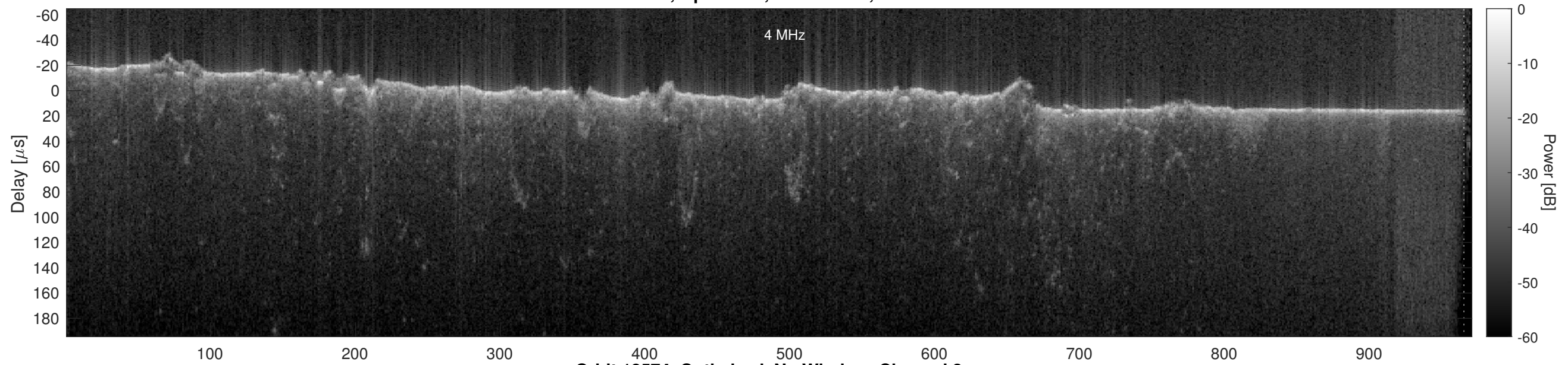
Orbit 18574, Optimized, No Window, Channel 2
