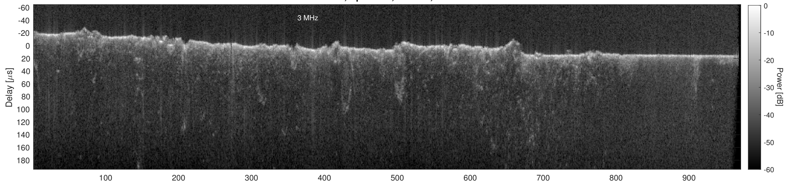
Orbit 18574, Cluttergram
