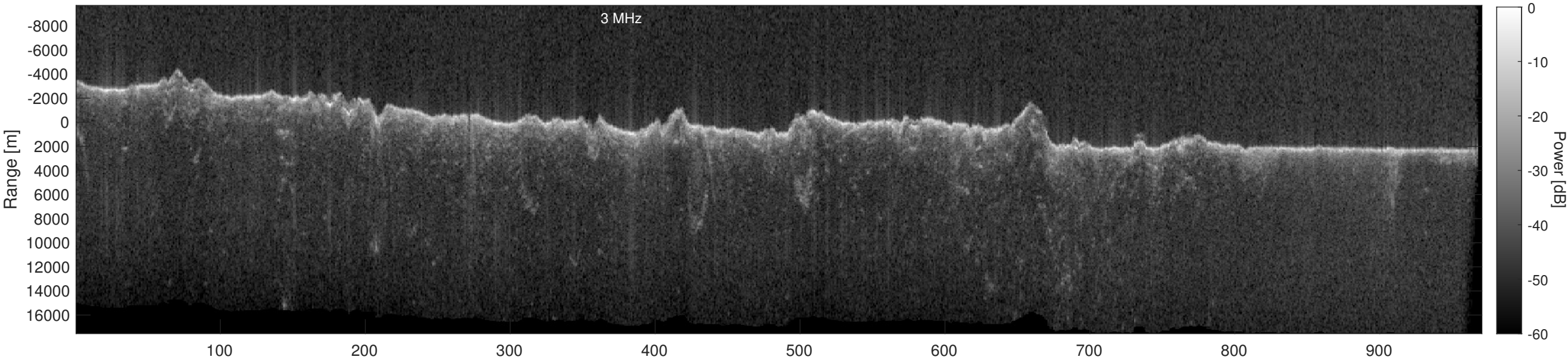
Orbit 18574, Depth-Corrected Cluttergram
