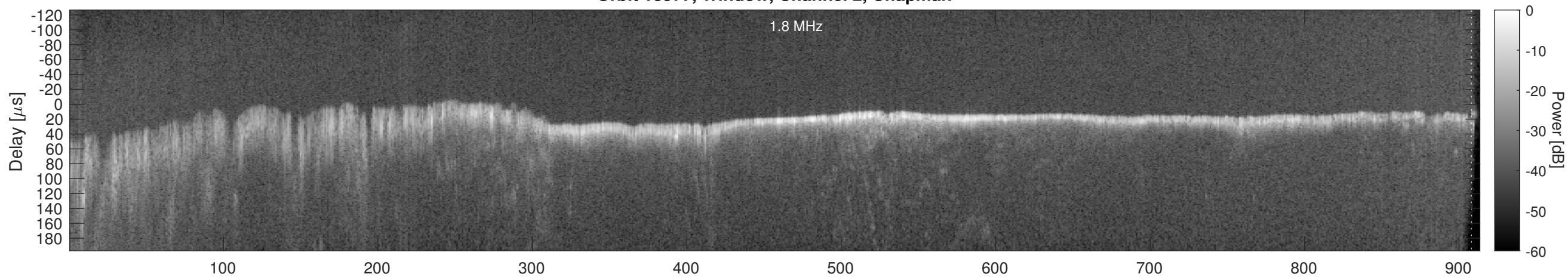
Orbit 18577, Window, Channel 2, Optimized
