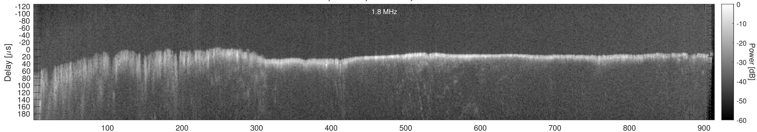
Orbit 18577, Window, Channel 2, Chapman
