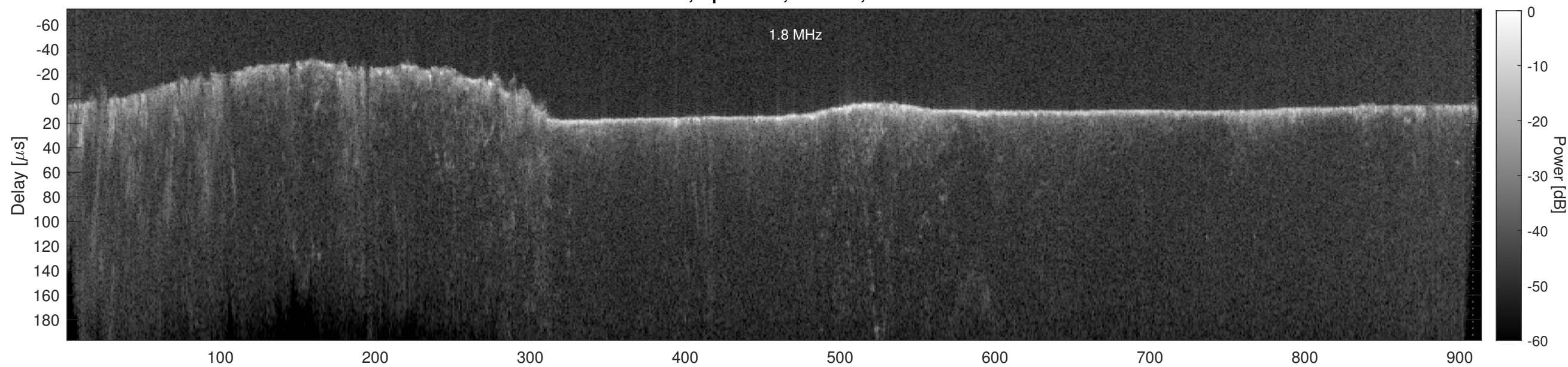
Orbit 18577, Cluttergram
