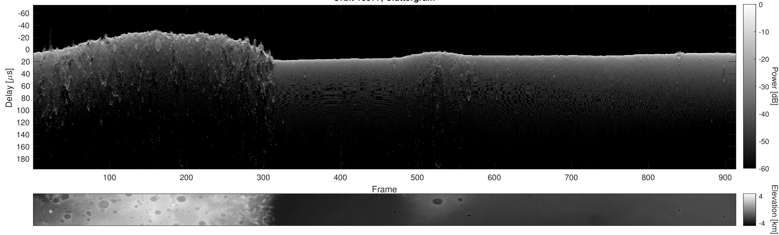
Orbit 18577, Cluttergram
