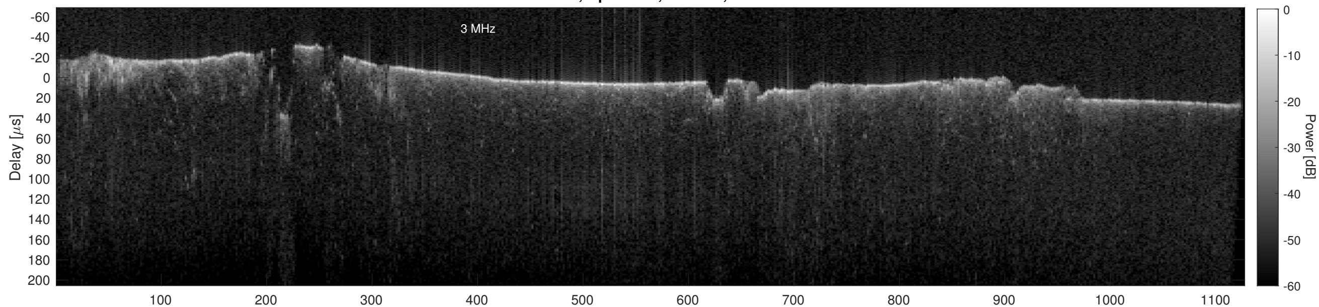
Orbit 18582, Cluttergram
