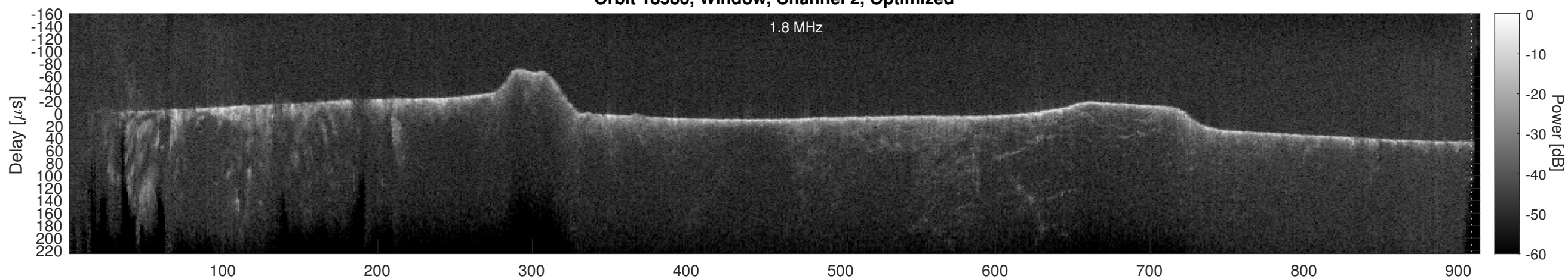
Orbit 18586, Cluttergram
