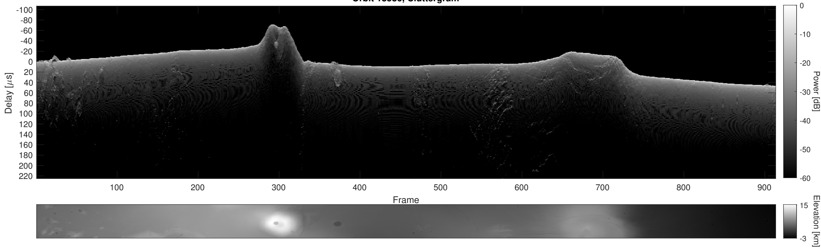
Orbit 18586, Cluttergram
