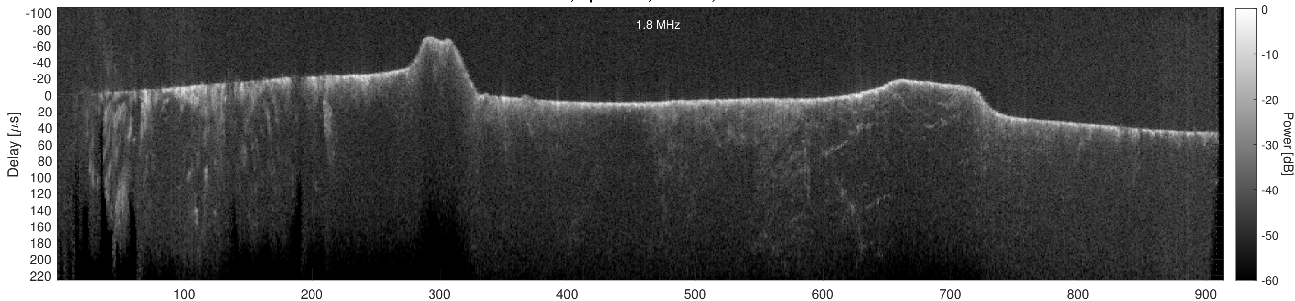
Orbit 18586, Cluttergram
