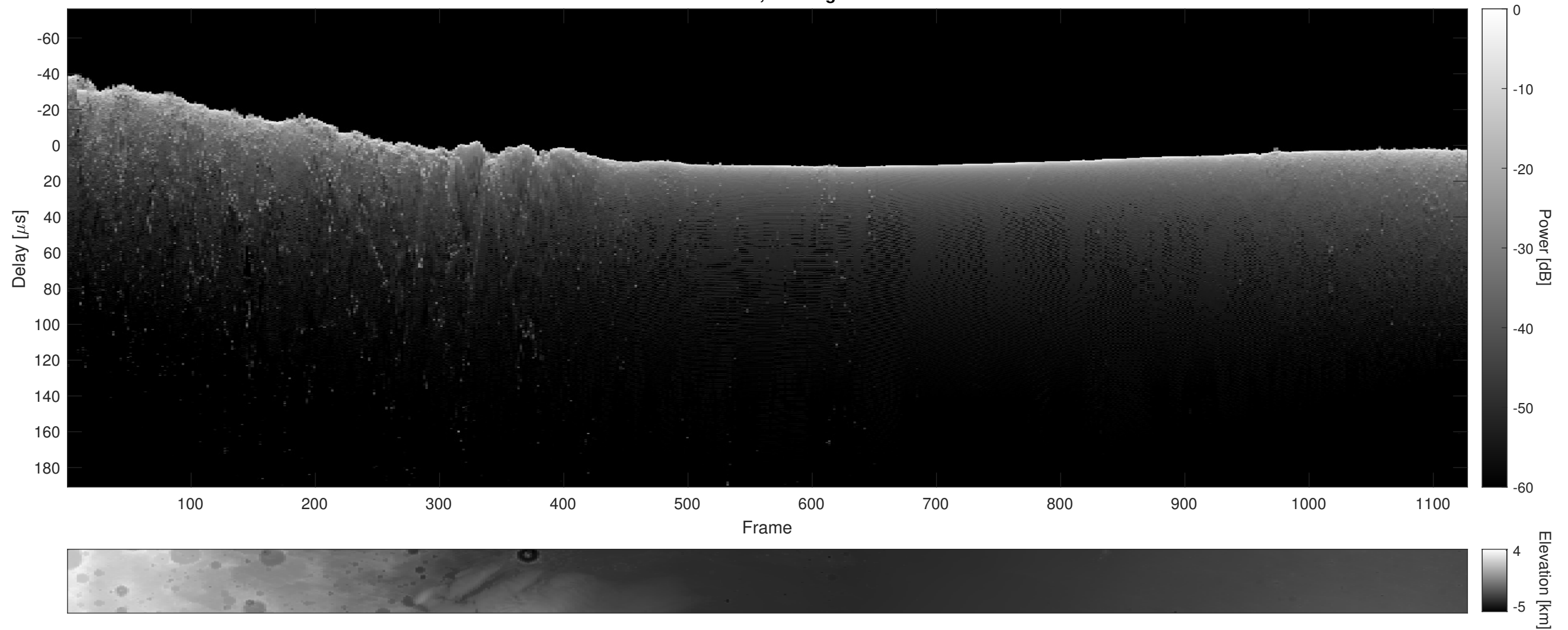
Orbit 18590, Cluttergram
