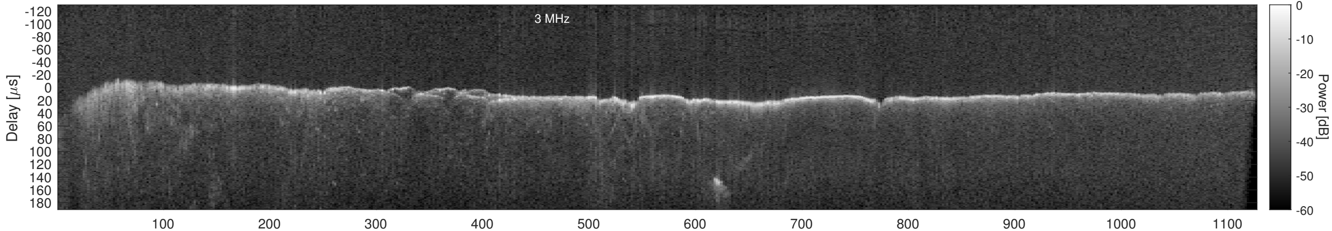
Orbit 18590, Window, Channel 2, Chapman
