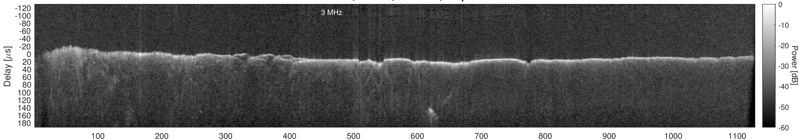
Orbit 18590, Window, Channel 2, Optimized
