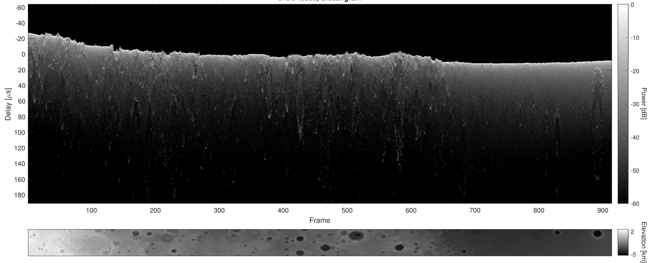
Orbit 18592, Cluttergram
