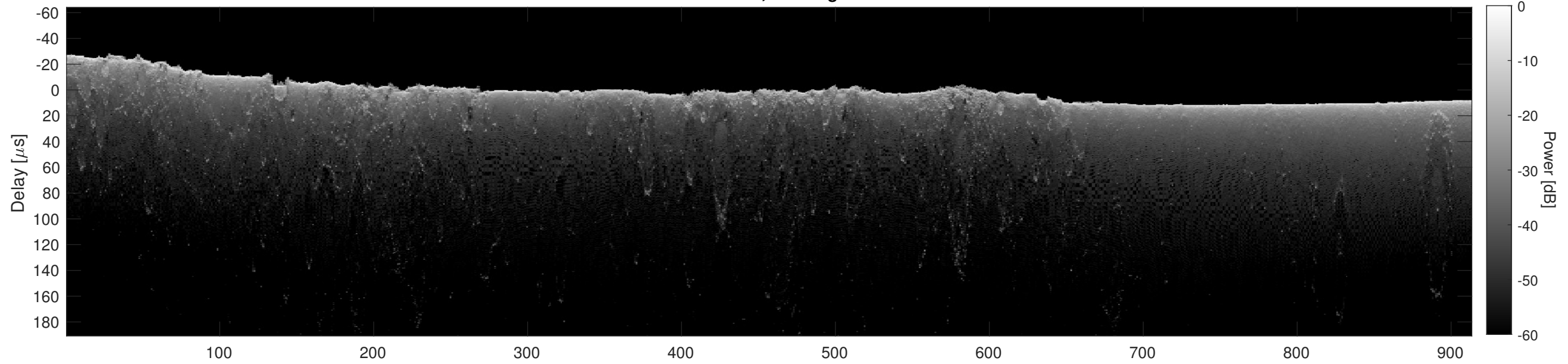
Orbit 18592, Cluttergram
