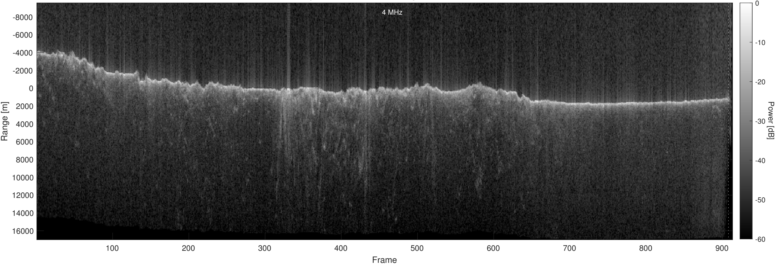
Orbit 18592, Optimized, No Window, Depth-Corrected, Channel 2
