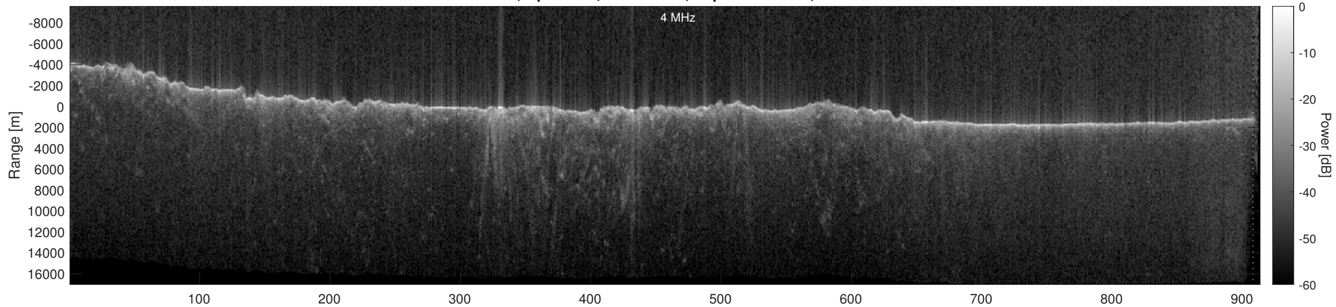
Orbit 18592, Optimized, No Window, Depth-Corrected, Channel 2
