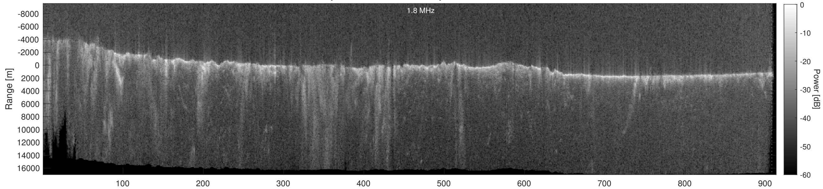
Orbit 18592, Depth-Corrected Cluttergram
