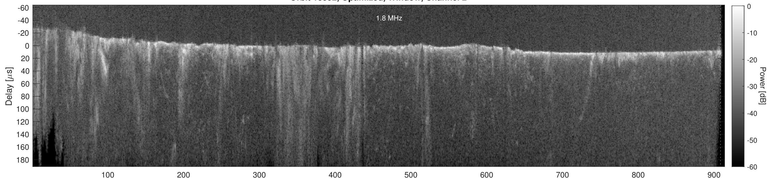
Orbit 18592, Cluttergram
