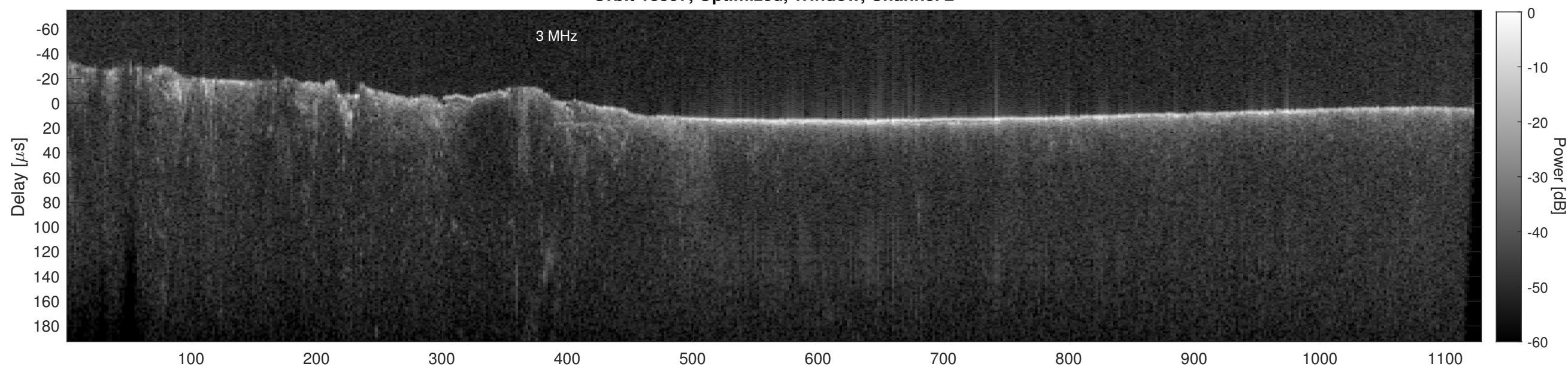
Orbit 18597, Cluttergram
