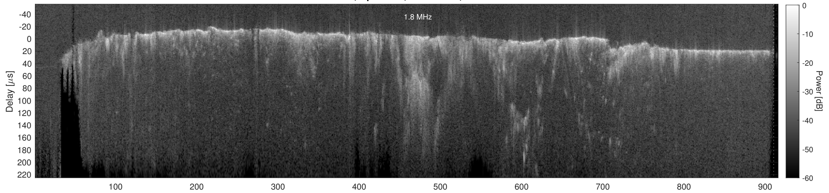
Orbit 18602, Cluttergram
